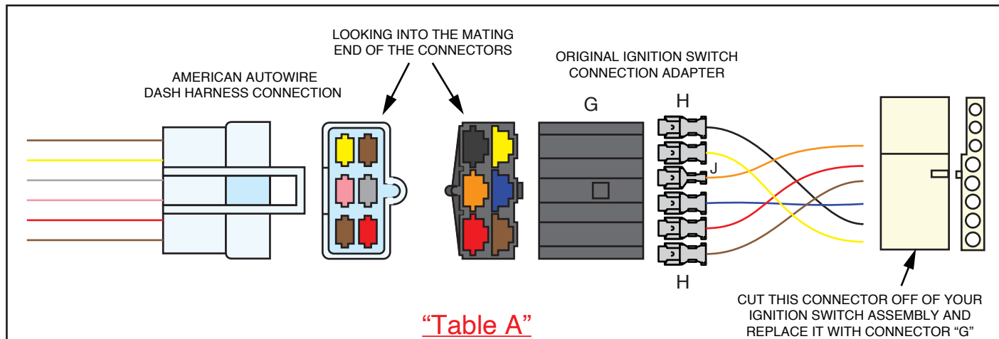
Mopar B-Body 1968-70 Ignition Switch Wires
