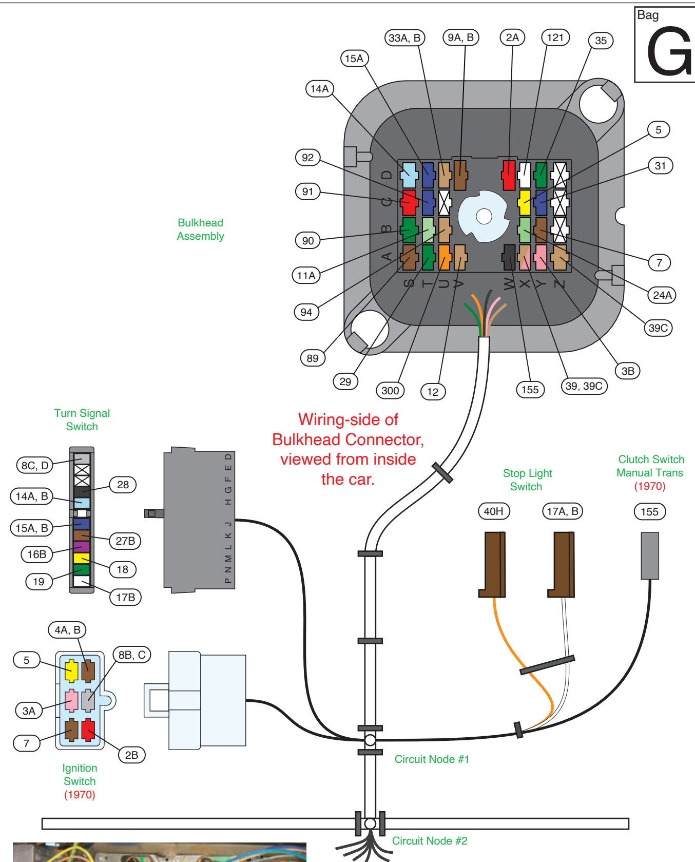
Circuit Node #2, at the center lower clip of the Instrument Panel
